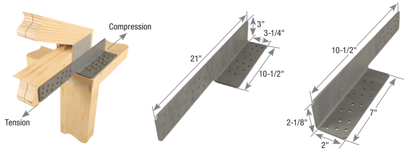
Typical DSC4R installation DSC4R right shown LDSC4L left shown
