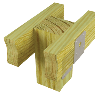
Typical SDJT14-TZ installation
