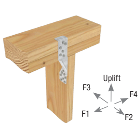
Typical TSP top plate installation (max nailing)
