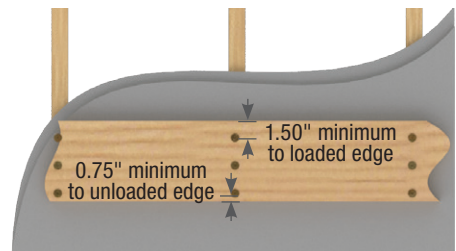
2x8 Detail
