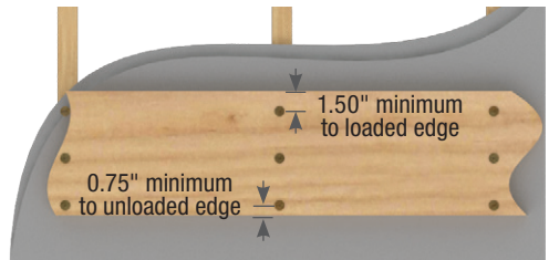
2x10 Detail
