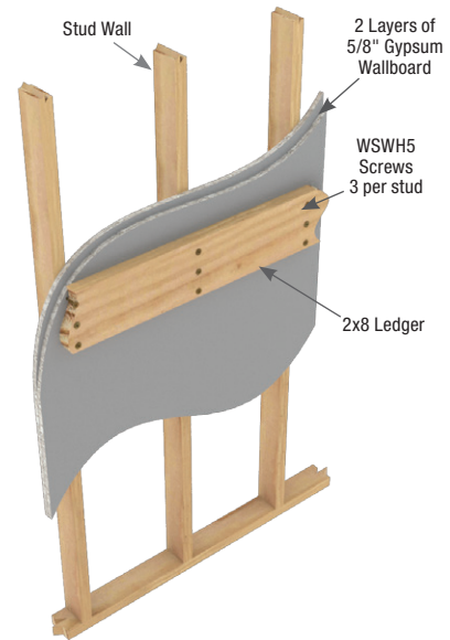
Typical 2x8 Ledger attached through 2 layers of 5/8" Gypsum Wallboard installation
