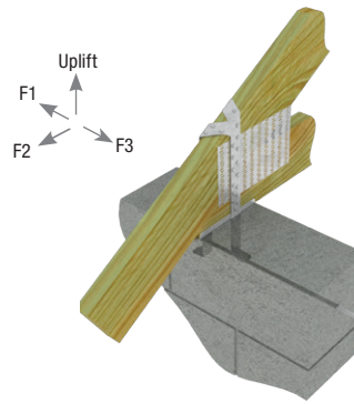
Typical DHTA 1-Ply installation
