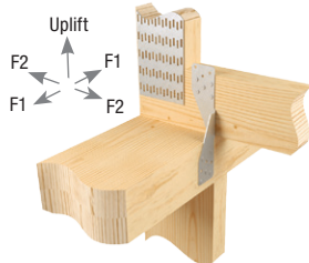
Typical RT7AT 2x4 bottom chord installation
