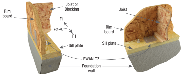
Offset Installation Typical FWAN-TZ offset max 4" from joist/blocking
