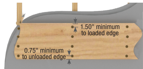
2x12 Detail
