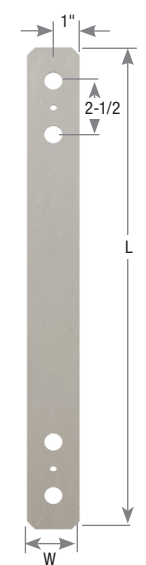
PS218-HDG PS418-HDG similar
