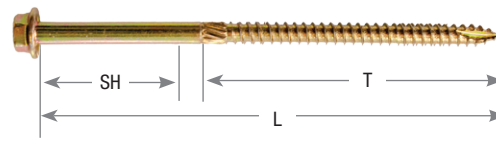
WS (Yellow Zinc finish)
