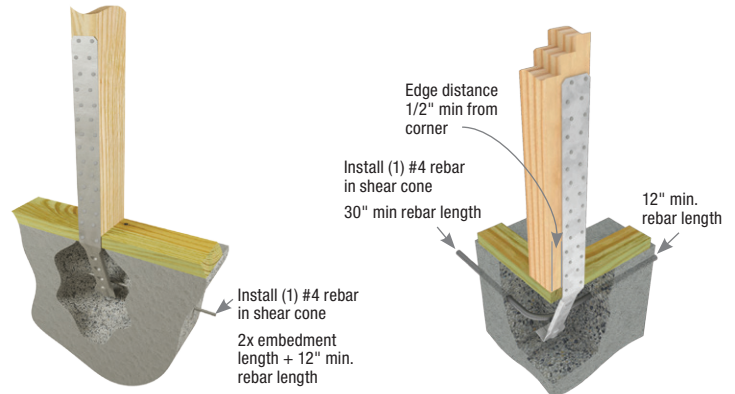
Typical STAD10 middle wall installation
