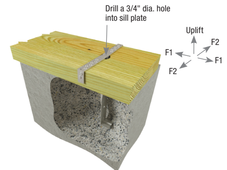
Alternate ST1-TZ installation with 3/4" center hole
