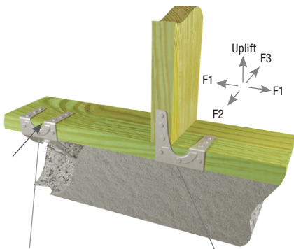
Typical FA4 standard installation
