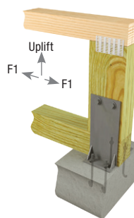
Typical SHA6T installation
