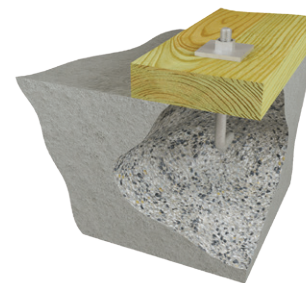
Typical Bearing Plate installation
