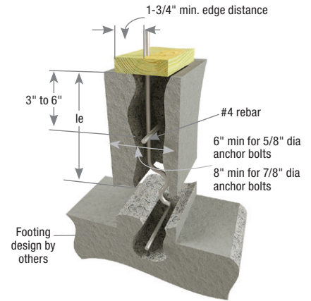
Typical STB anchor bolt installation
