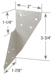
RT4 (left version shown)
