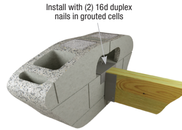
Typical MPH double-ply installation
