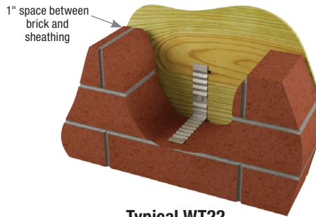
Typical WT22 installation
