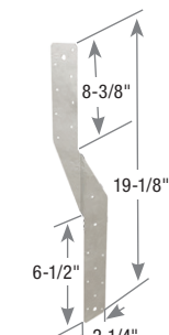
LFTA6 (left version shown)
