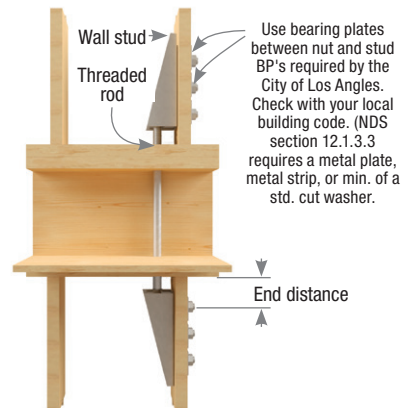
Holdown installation between floors
