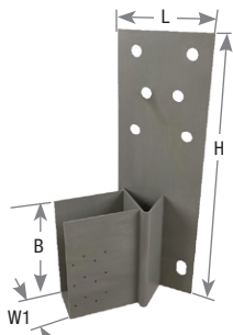
GT skewed
