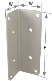
ML26-TZ (ML24-TZ similar)
