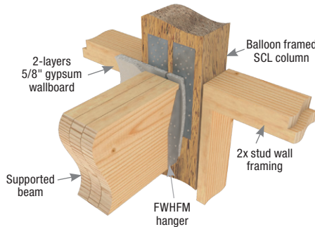
Typical FWHFM installation
