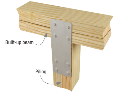
Typical PS720-HDG installation
