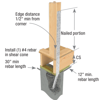
Typical STAD14RJ corner rim joist installation
