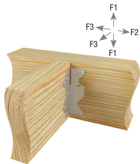
Typical MPA1 joist / header installation
