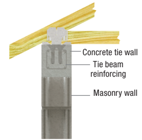
Typical HLPTA75 double rebar installation
