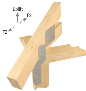
Typical LUGTC2 corner hip installation
