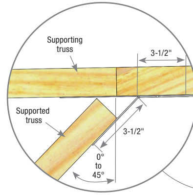
Alternate SNP3 installation Figure 2
