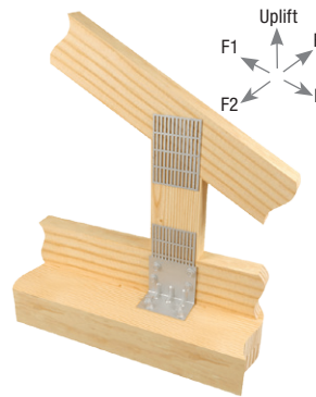
Typical HGA10 installation
