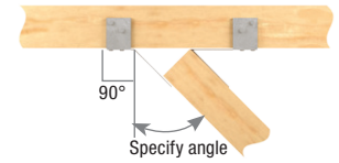
Typical HDO hanger skewed, right shown (square cut)
