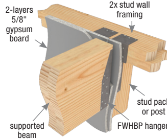
Typical FWHBP attachment to top plate/beam and stud pack/post
