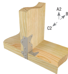
Typical MPA1 stud / plate installation
