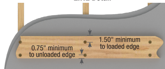
2x6 Detail
