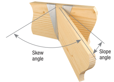
Typical BPH hanger sloped down, skewed right, low side flush shown
