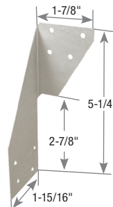
RT5 (left version shown)
