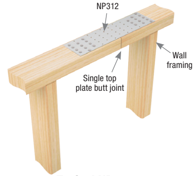
Typical NP312 IRC prescriptive top plate splice installation
