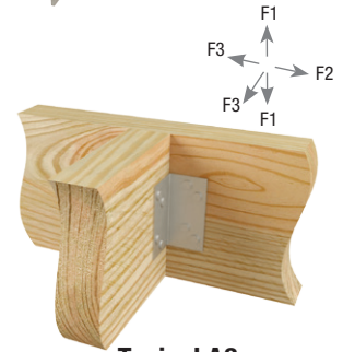
Typical A3 installation
