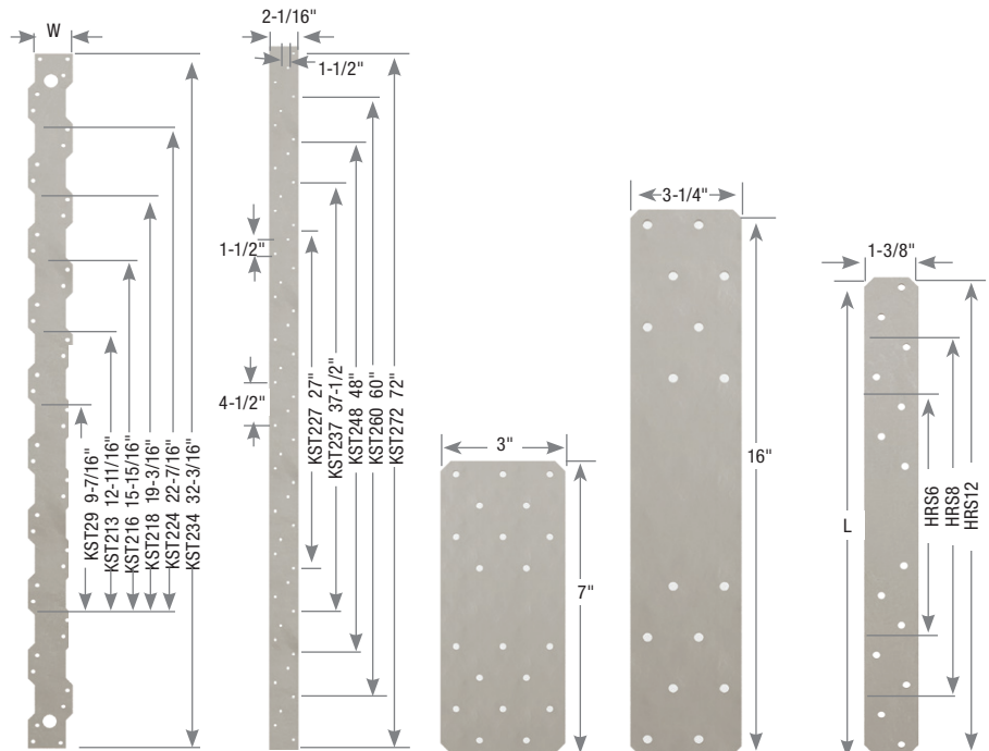
KST scalloped design
