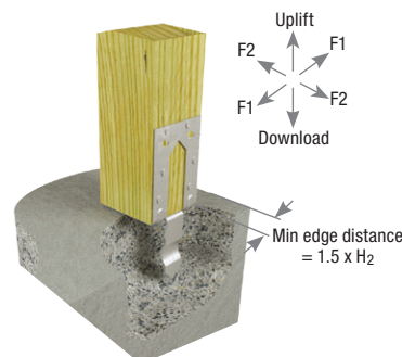
Typical WE installation
