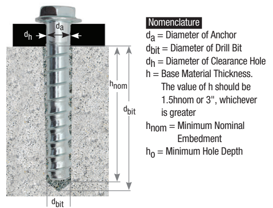
Screw-Bolt™ + anchor detail
