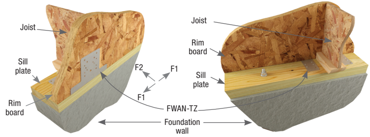
Centered Installation Typical FWAN-TZ centered on joist/blocking
