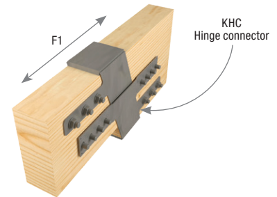
Typical KHCST installation
