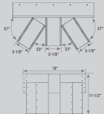
Custom Order EXAMPLE: HLBH 3 pocket Girder Truss Hanger
