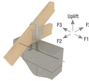
Typical HHTA20 double roof-truss installation
