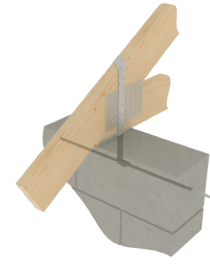
Typical HHTA20 single roof-truss installation
