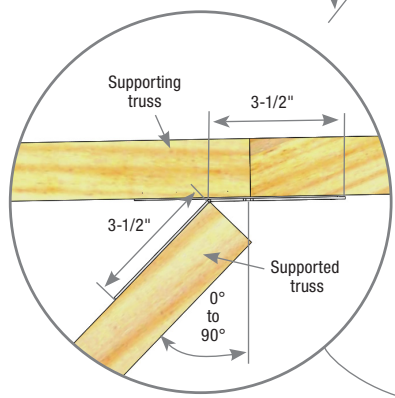
Typical SNP3 installation Figure 1
