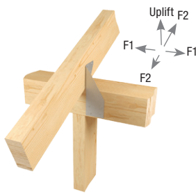
Typical RT5 truss/rafter to double plate installation
