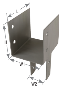
Optional KECC rotated straps 90°
