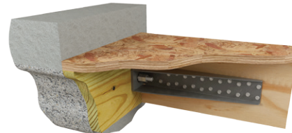
Typical UPHD concrete wall installation
