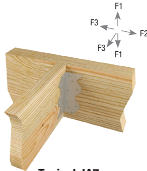
Typical JA7 installation
