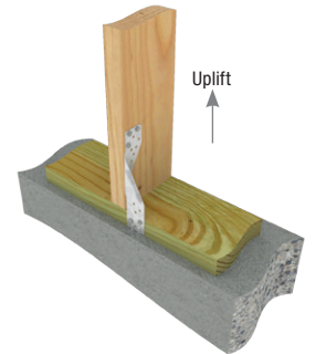
Typical TSP-TZ mudsill installation (min nailing)
