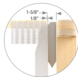
Figure 1 Typical FWH Side View
