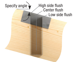
Typical BPH hanger sloped top flange right shown (this configuration will not be open back)
