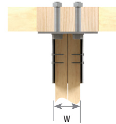
GT top view
