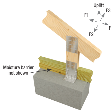
Typical HGAM10 installation
