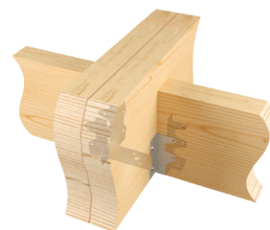
Typical DTUS24 installation
