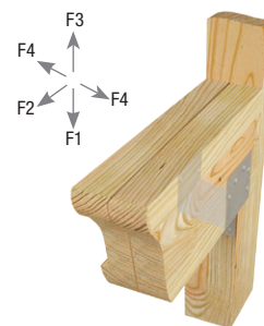
Typical HH44 installation
