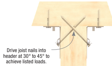
Typical THDH double shear installation
