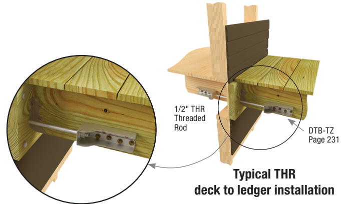
Typical THR installation
