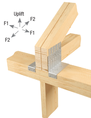
Typical SBP installation
