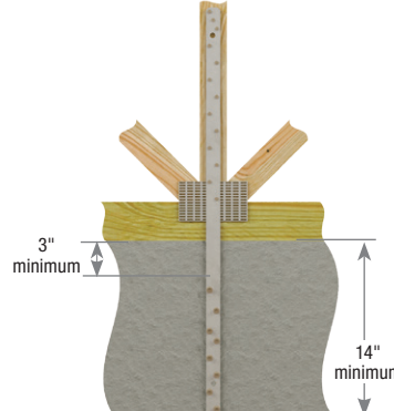
Typical MSTAM36 installation
