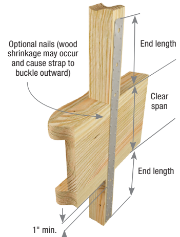
Typical KST237 floor-to-floor installation
