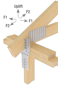
Typical LUGT1 installation
