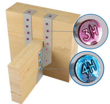
Typical MiTek hanger installation using TECO 33° Collated Nails
